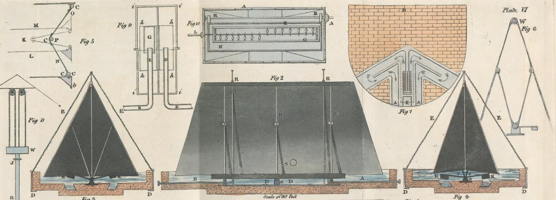
Gas Holder at Westminster Without Specific Gravity Apparatus. Capacity 15,400 Cubic Feet.
