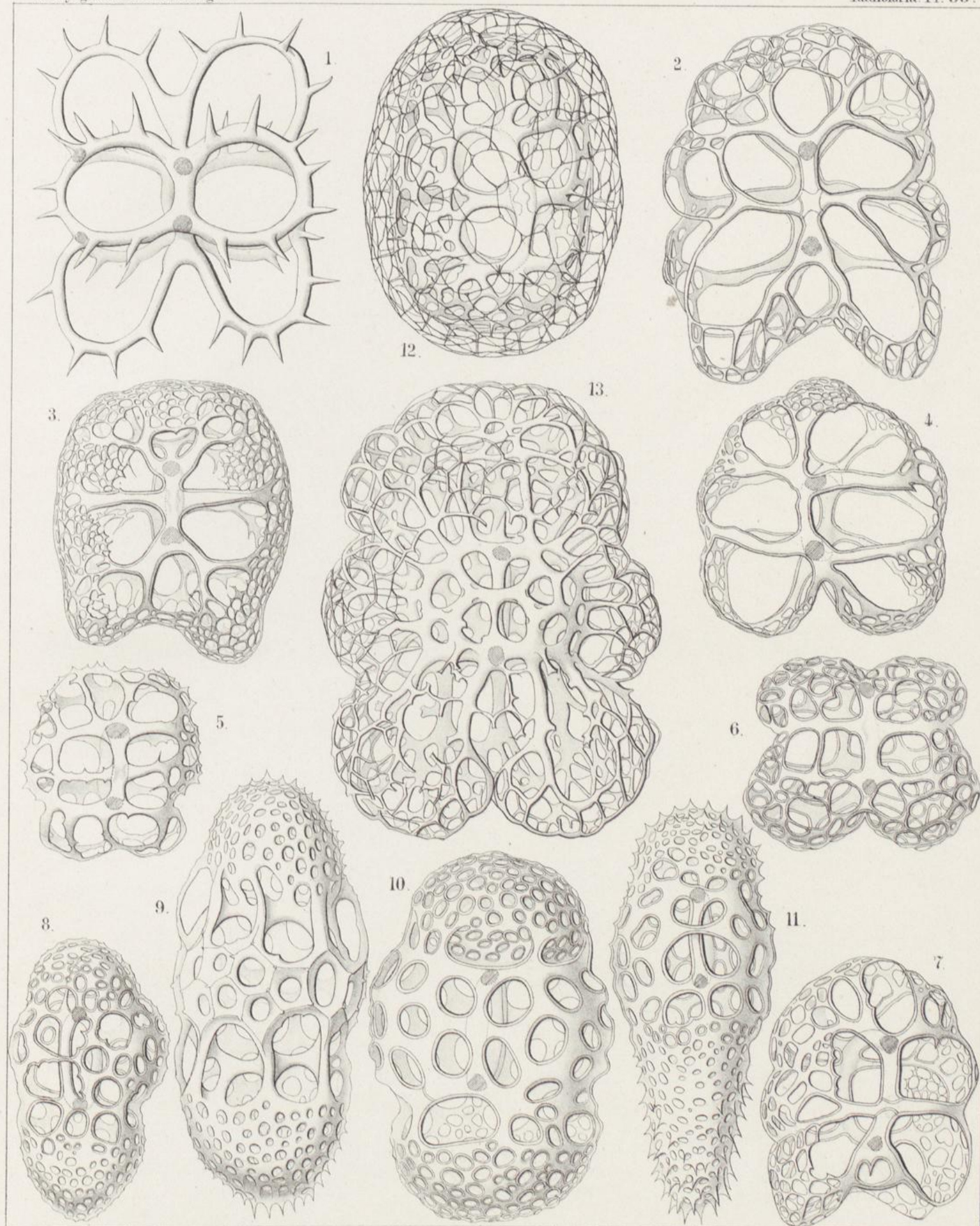
1. CIRCOSPYRIS, 2-7. AMPHISPYRIS, 8-11. TRICOLOSPYRIS, 12 13. PERISPYRIS.
